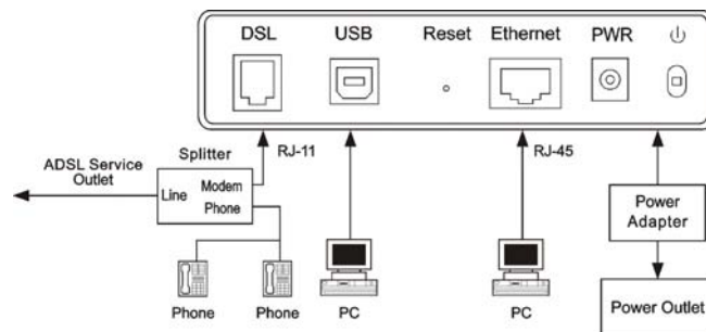
Figure 3.2-1 ZXDSL 831A II Connection Schematic Diagram (No Phone sets are Installed Before the Splitter)
