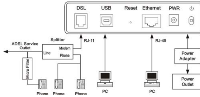
Figure 3.2-2 ZXDSL 831A II Connection Schematic Diagram (Phone sets are Installed Before the Splitter)
